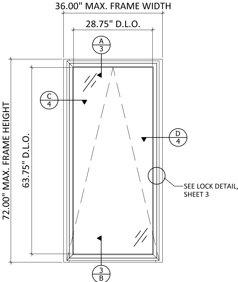
PROJECT OUT WINDOW ELEVATION EXTERIOR ELEVATION VIEW
