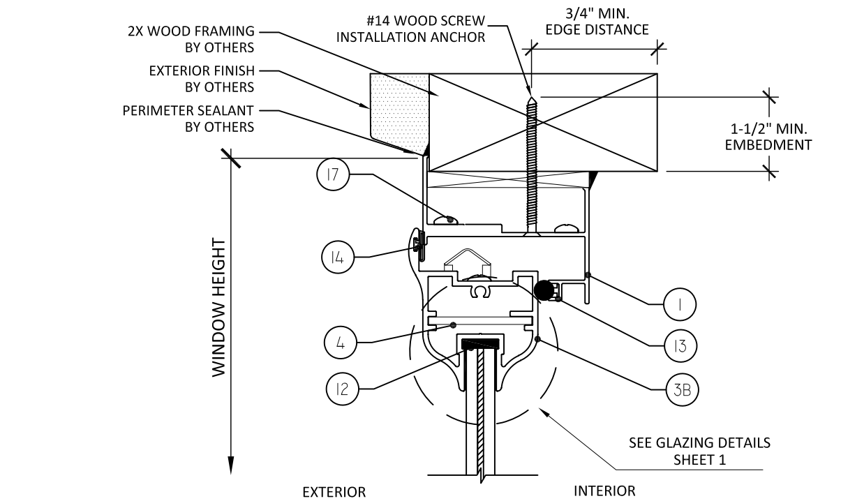
A 3 VERTICAL SECTION HEAD - 2X WOOD FRAME
